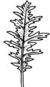
INCISED
