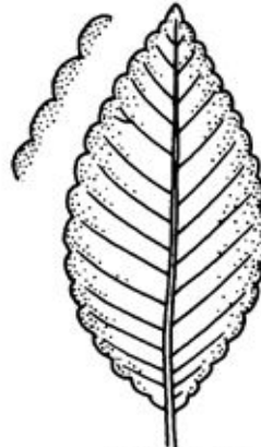
CRENATE
