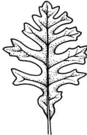
CLEFT
