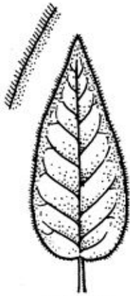
CILIATE
